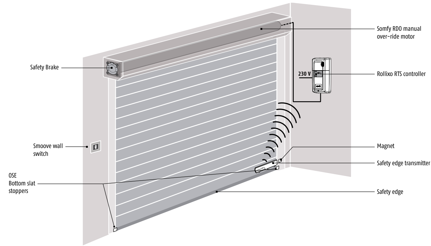
Illustration of a Rollixo RTS installation with a wireless optical safety edge system.
